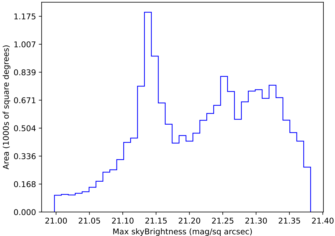
ddf_loaded_fl15_v3.4_10yrs WFD r band: Max skyBrightness
