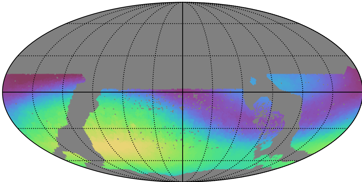
ddf_loaded_fl15_v3.4_10yrs WFD g band: Max skyBrightness
