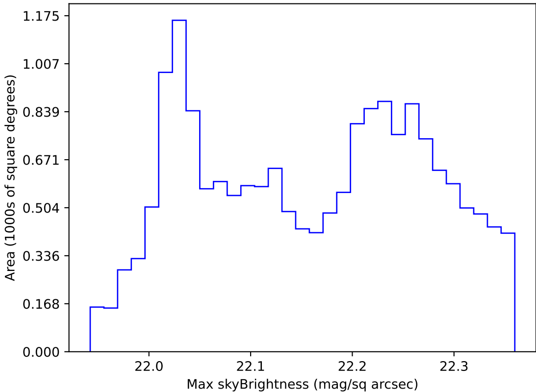
ddf_loaded_fl15_v3.4_10yrs WFD g band: Max skyBrightness
