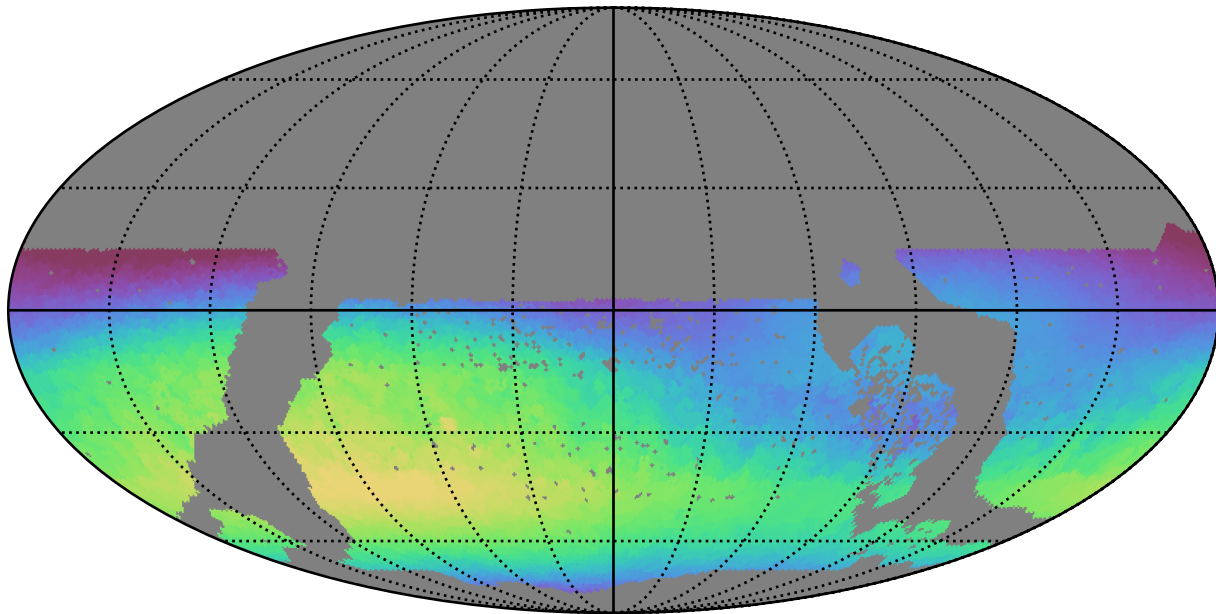
ddf_loaded_fl15_v3.4_10yrs WFD all bands: Max skyBrightness
