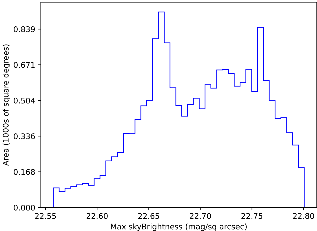
ddf_loaded_fl15_v3.4_10yrs WFD all bands: Max skyBrightness
