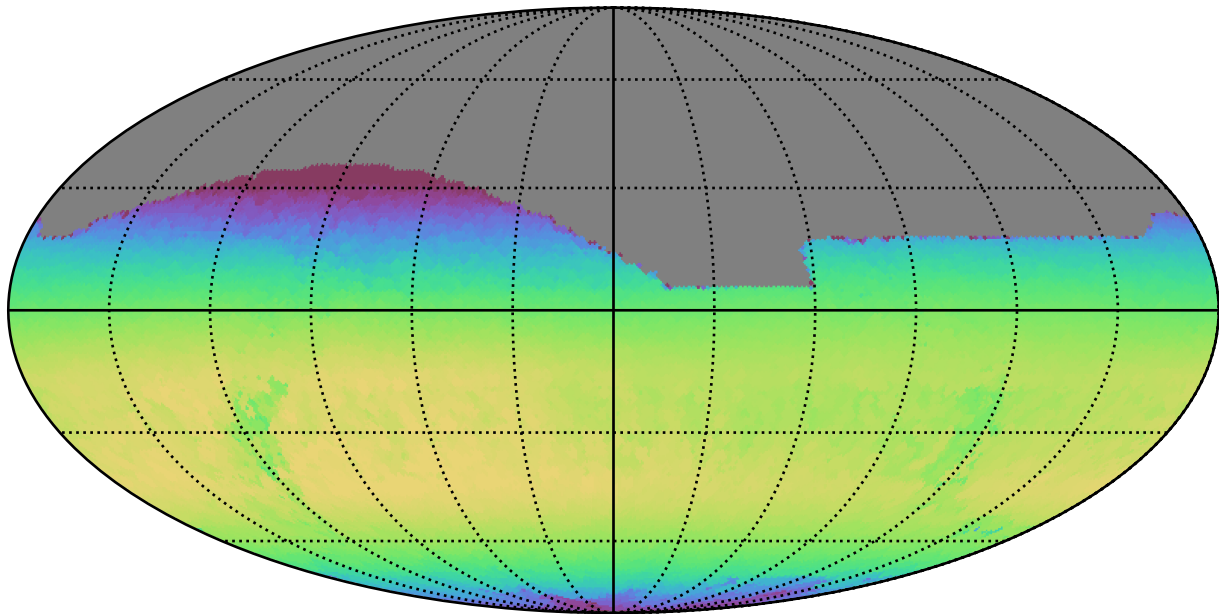
ddf_loaded_fl15_v3.4_10yrs All sky z band: Max skyBrightness
