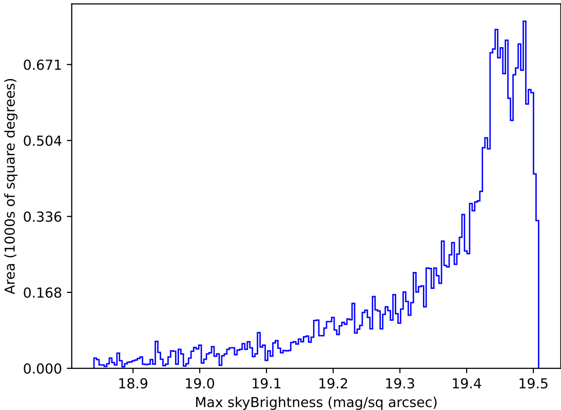
ddf_loaded_fl15_v3.4_10yrs All sky z band: Max skyBrightness
