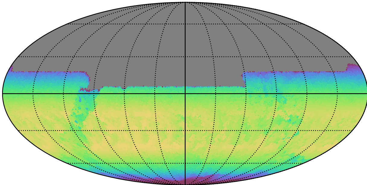
ddf_loaded_fl15_v3.4_10yrs All sky y band: Max skyBrightness
