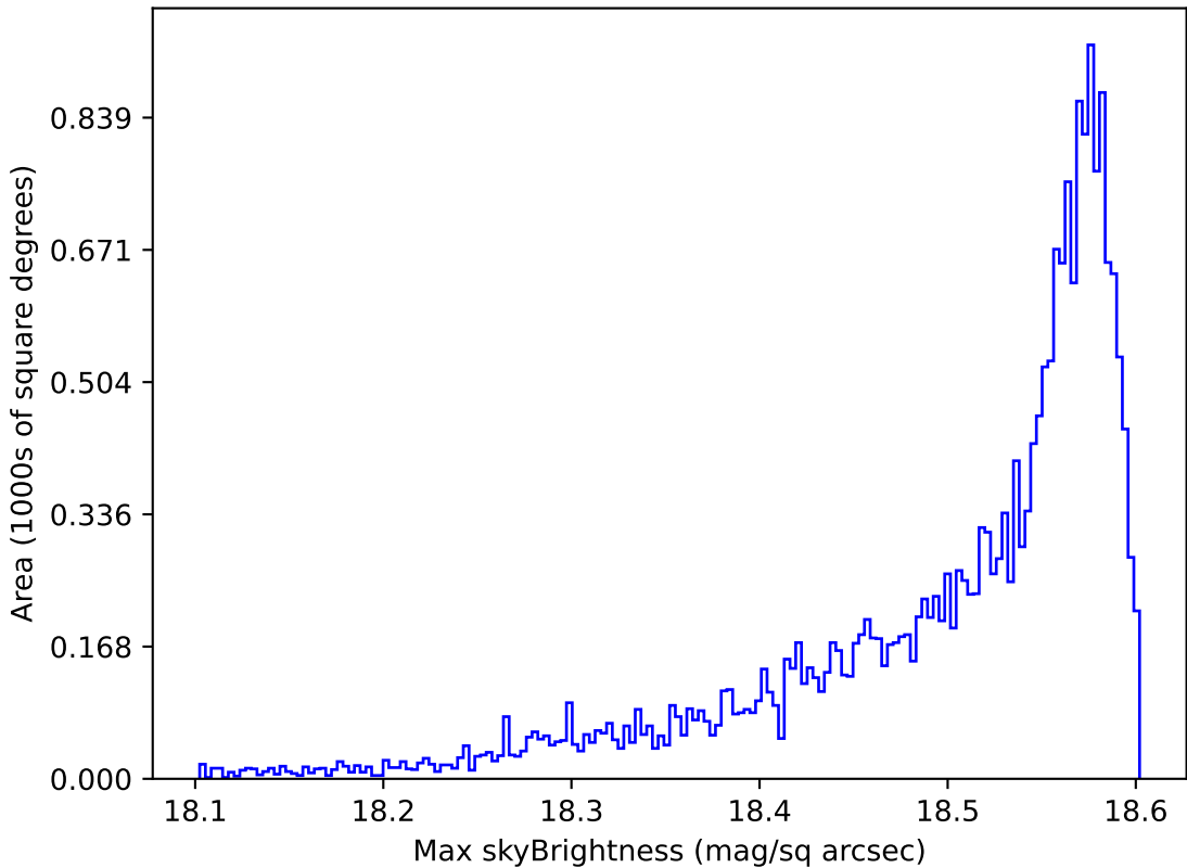
ddf_loaded_fl15_v3.4_10yrs All sky y band: Max skyBrightness
