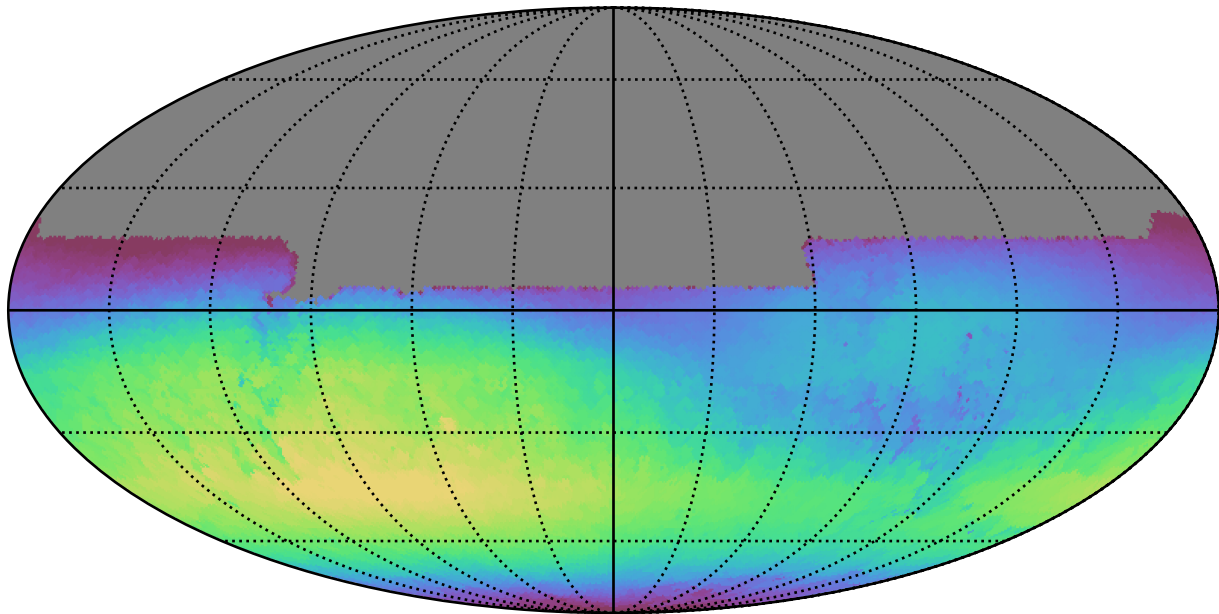
ddf_loaded_fl15_v3.4_10yrs All sky u band: Max skyBrightness
