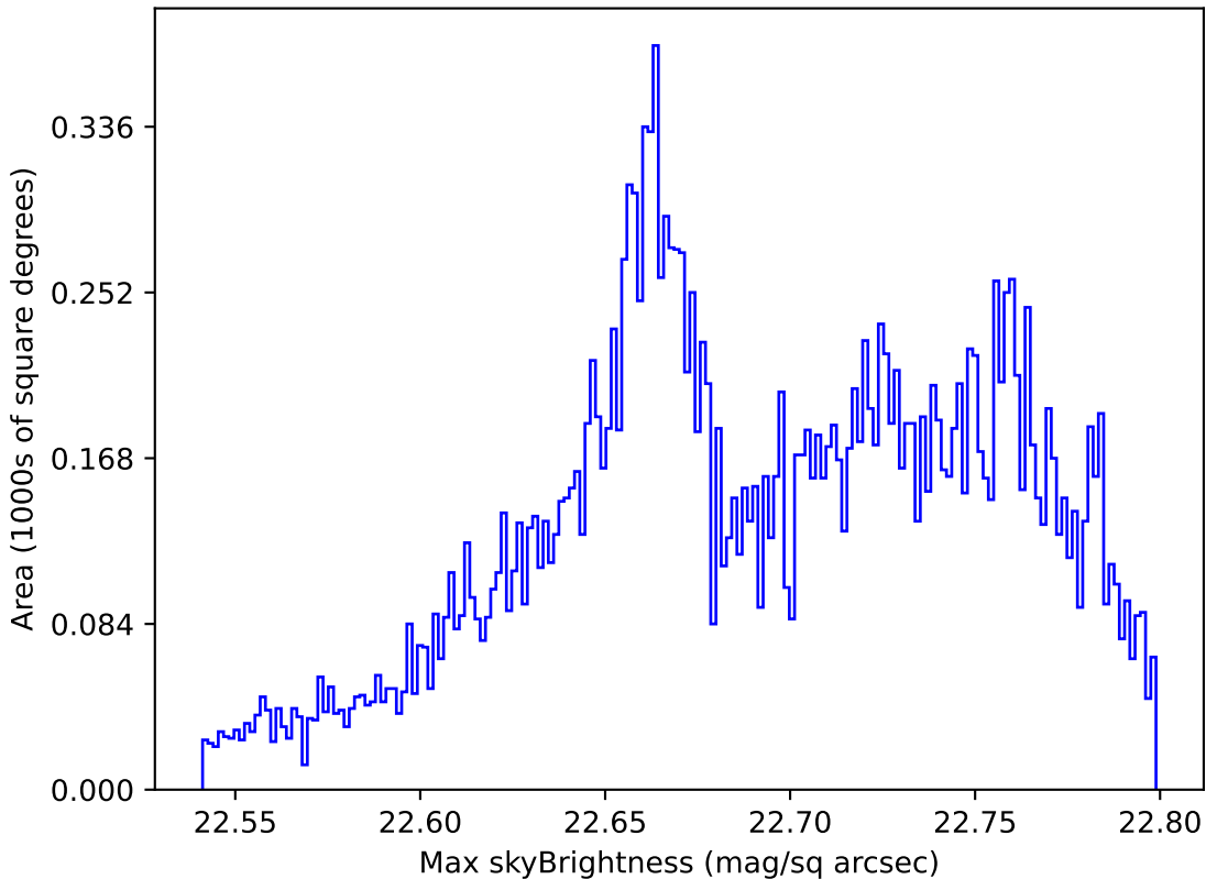
ddf_loaded_fl15_v3.4_10yrs All sky u band: Max skyBrightness
