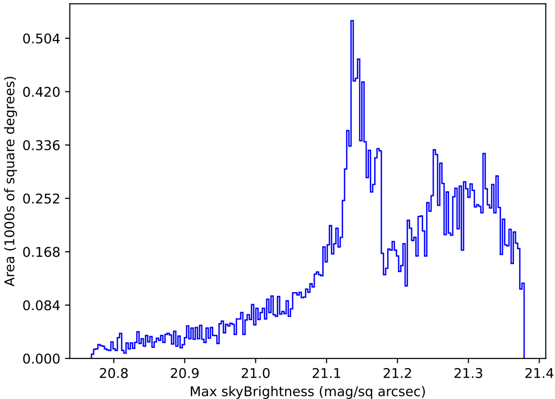
ddf_loaded_fl15_v3.4_10yrs All sky r band: Max skyBrightness
