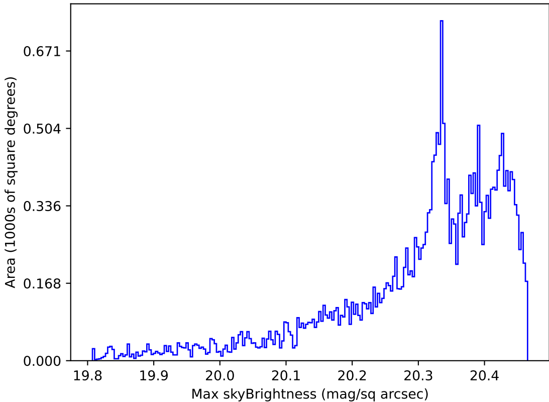
ddf_loaded_fl15_v3.4_10yrs All sky i band: Max skyBrightness
