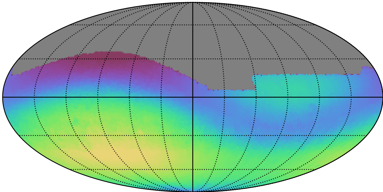
ddf_loaded_fl15_v3.4_10yrs All sky g band: Max skyBrightness
