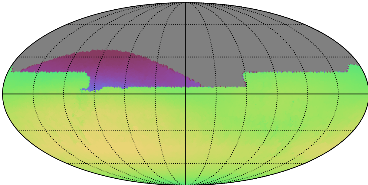
ddf_loaded_fl15_v3.4_10yrs All sky all bands: Max skyBrightness
