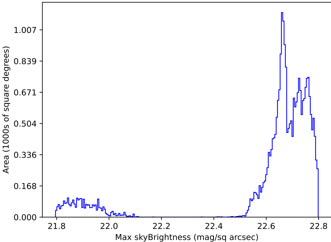
ddf_loaded_fl15_v3.4_10yrs All sky all bands: Max skyBrightness
