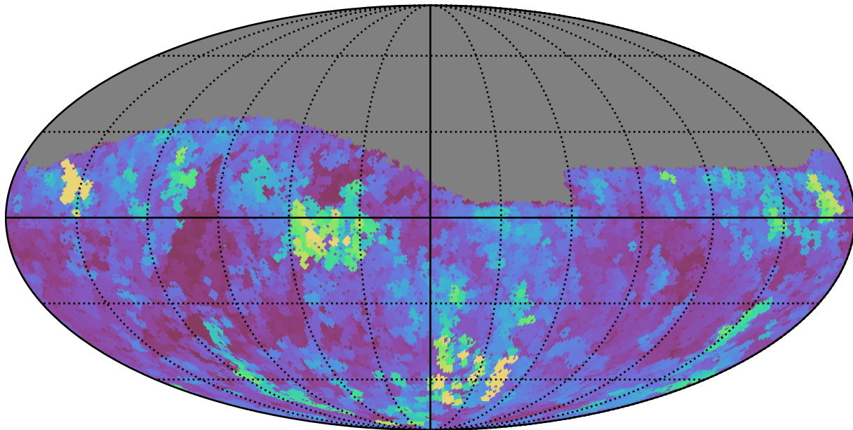
ddf_loaded_fl15_v3.4_10yrs Yr 1 z band: Max seeingGeom
