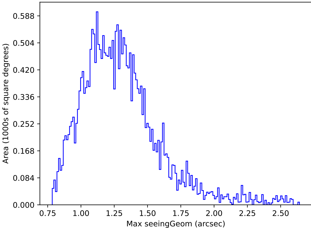
ddf_loaded_fl15_v3.4_10yrs Yr 1 z band: Max seeingGeom
