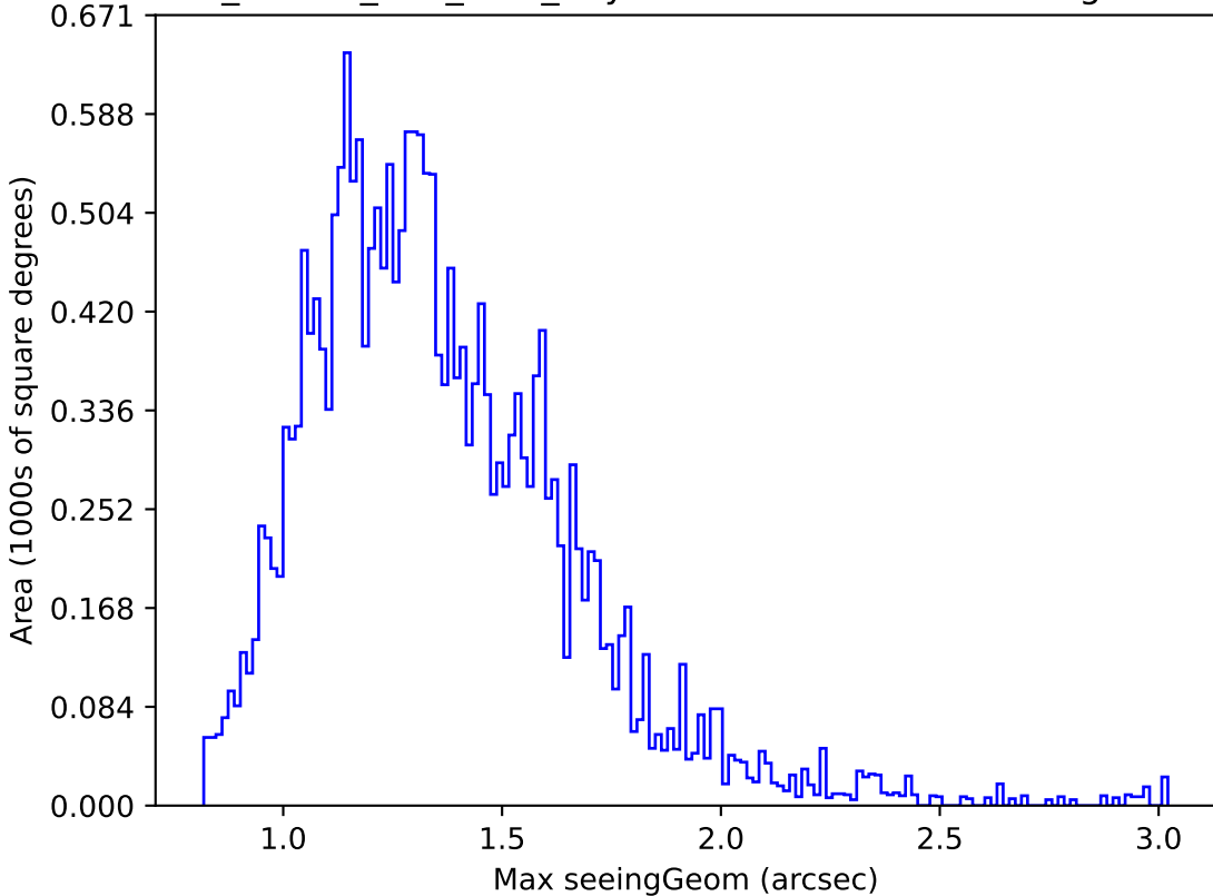
ddf_loaded_fl15_v3.4_10yrs Yr 1 u band: Max seeingGeom
