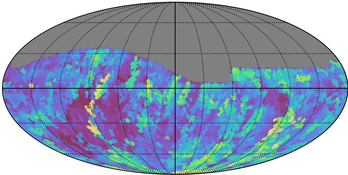
ddf_loaded_fl15_v3.4_10yrs Yr 1 r band: Max seeingGeom
