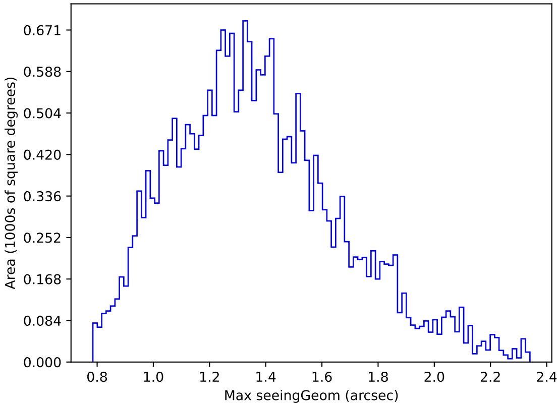
ddf_loaded_fl15_v3.4_10yrs Yr 1 r band: Max seeingGeom
