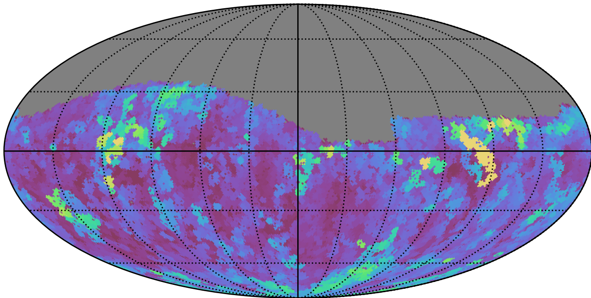
ddf_loaded_fl15_v3.4_10yrs Yr 1 g band: Max seeingGeom
