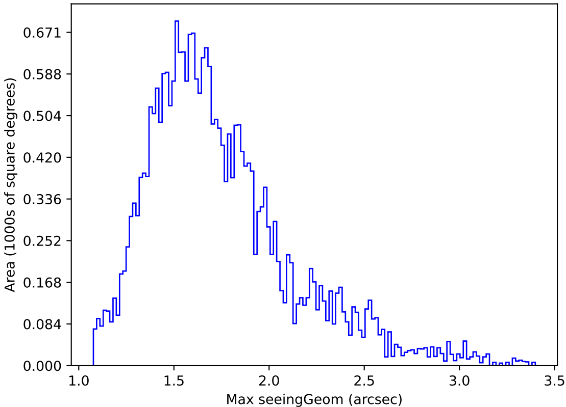
ddf_loaded_fl15_v3.4_10yrs Yr 1 all bands: Max seeingGeom
