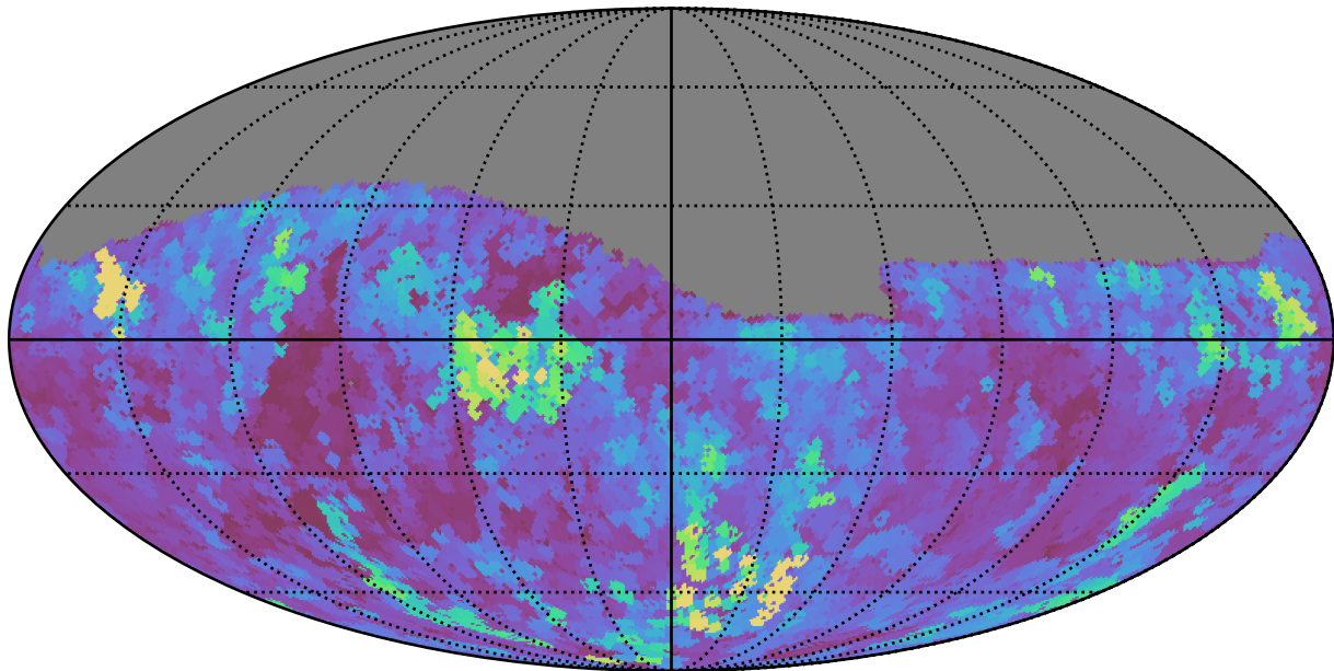
ddf_loaded_fl15_v3.4_10yrs Yr 1 z band: Max seeingEff
