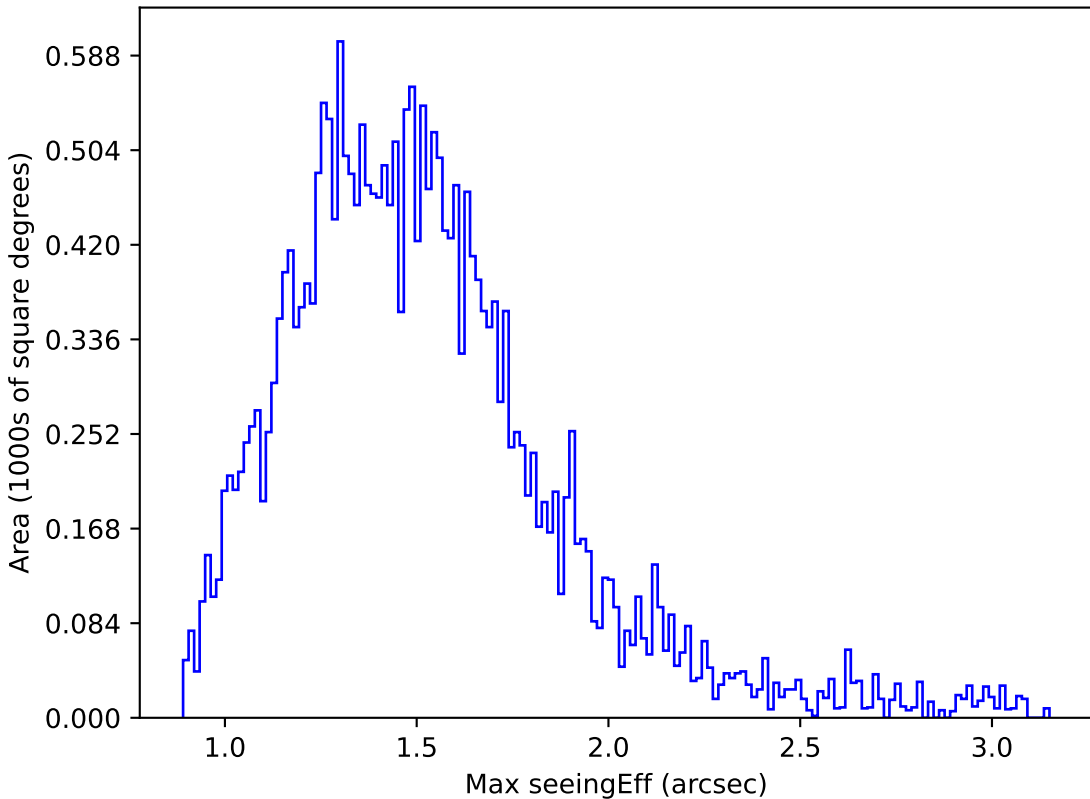
ddf_loaded_fl15_v3.4_10yrs Yr 1 z band: Max seeingEff
