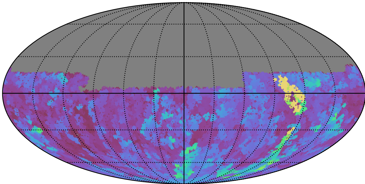
ddf_loaded_fl15_v3.4_10yrs Yr 1 u band: Max seeingEff
