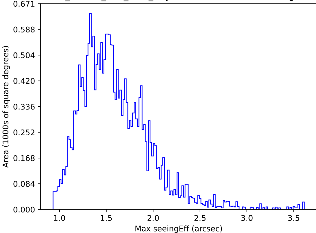
ddf_loaded_fl15_v3.4_10yrs Yr 1 u band: Max seeingEff
