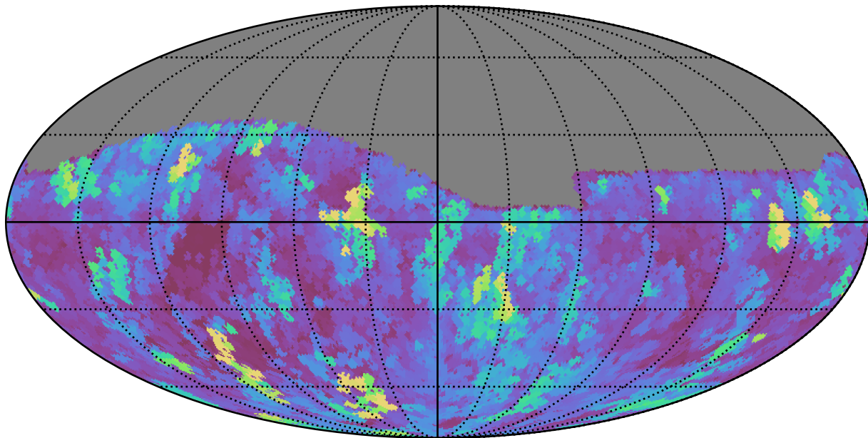
ddf_loaded_fl15_v3.4_10yrs Yr 1 i band: Max seeingEff
