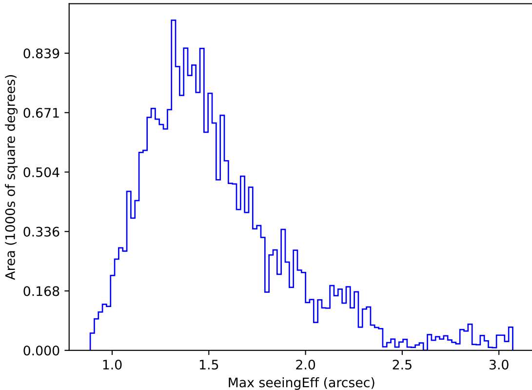
ddf_loaded_fl15_v3.4_10yrs Yr 1 i band: Max seeingEff
