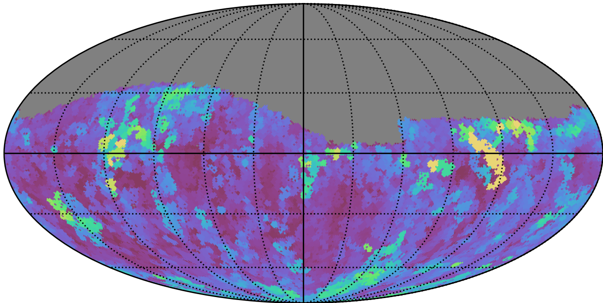
ddf_loaded_fl15_v3.4_10yrs Yr 1 g band: Max seeingEff
