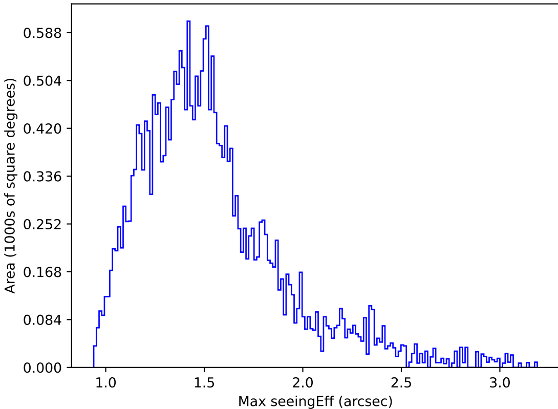
ddf_loaded_fl15_v3.4_10yrs Yr 1 g band: Max seeingEff
