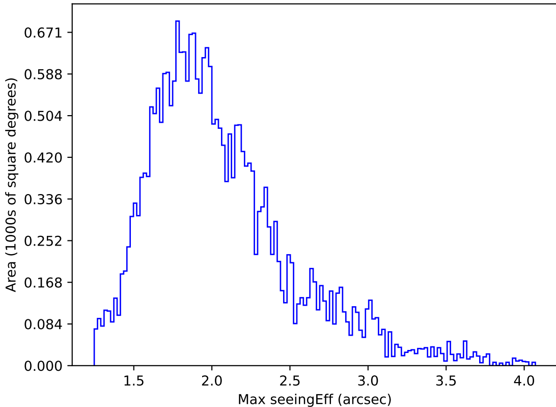
ddf_loaded_fl15_v3.4_10yrs Yr 1 all bands: Max seeingEff
