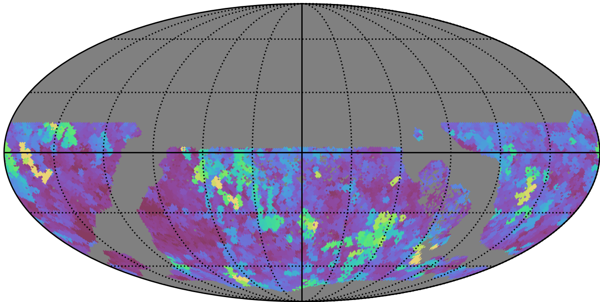
ddf_loaded_fl15_v3.4_10yrs WFD z band: Max seeingEff
