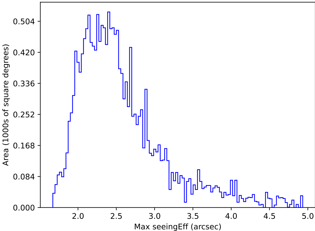
ddf_loaded_fl15_v3.4_10yrs WFD z band: Max seeingEff
