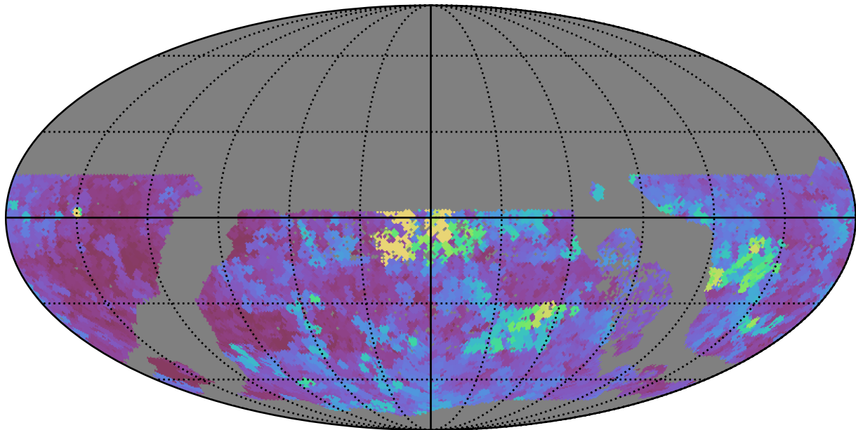
ddf_loaded_fl15_v3.4_10yrs WFD y band: Max seeingEff
