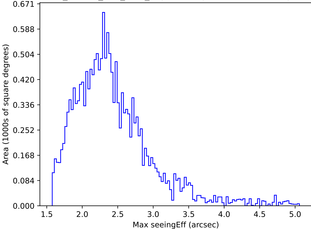
ddf_loaded_fl15_v3.4_10yrs WFD y band: Max seeingEff
