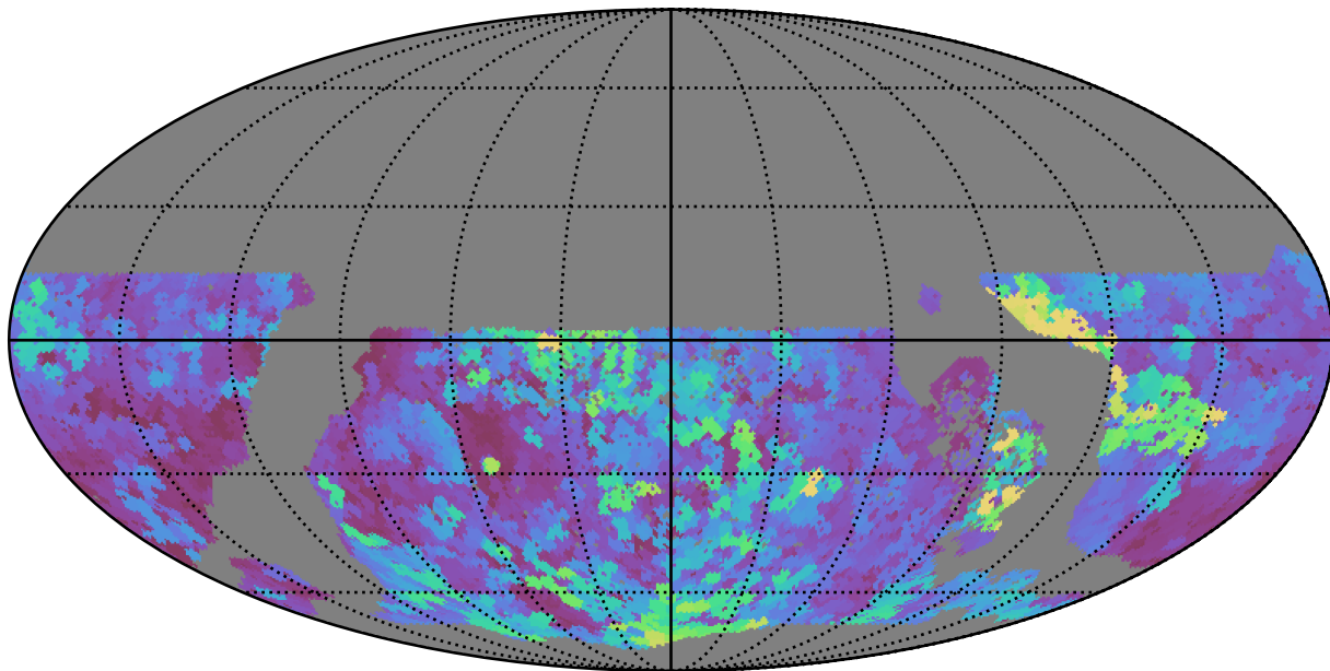
ddf_loaded_fl15_v3.4_10yrs WFD u band: Max seeingEff
