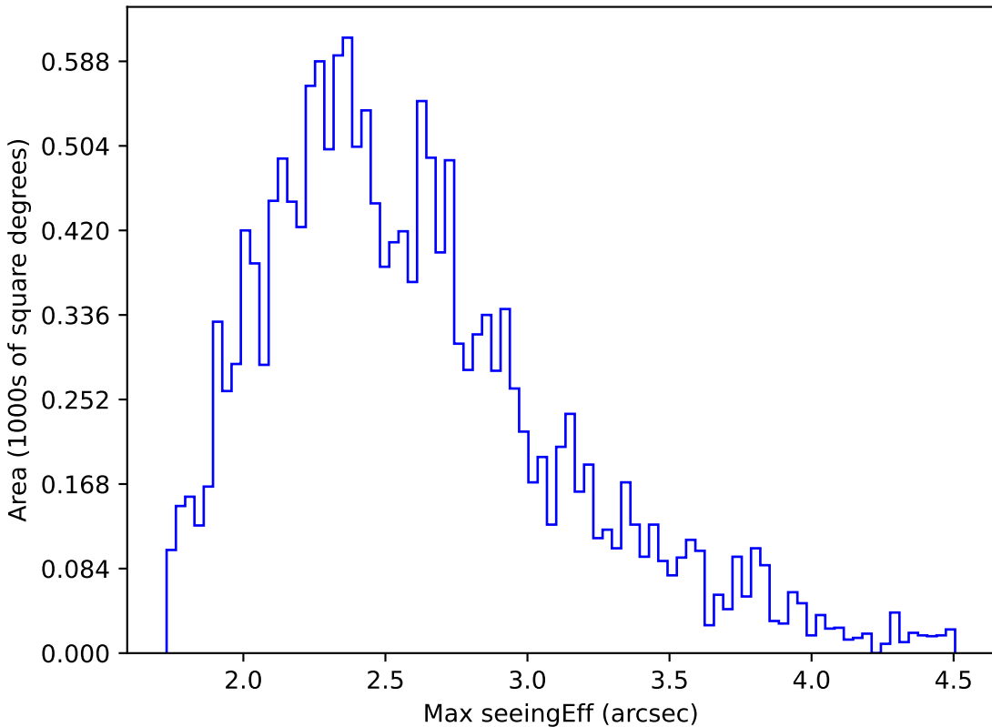
ddf_loaded_fl15_v3.4_10yrs WFD u band: Max seeingEff
