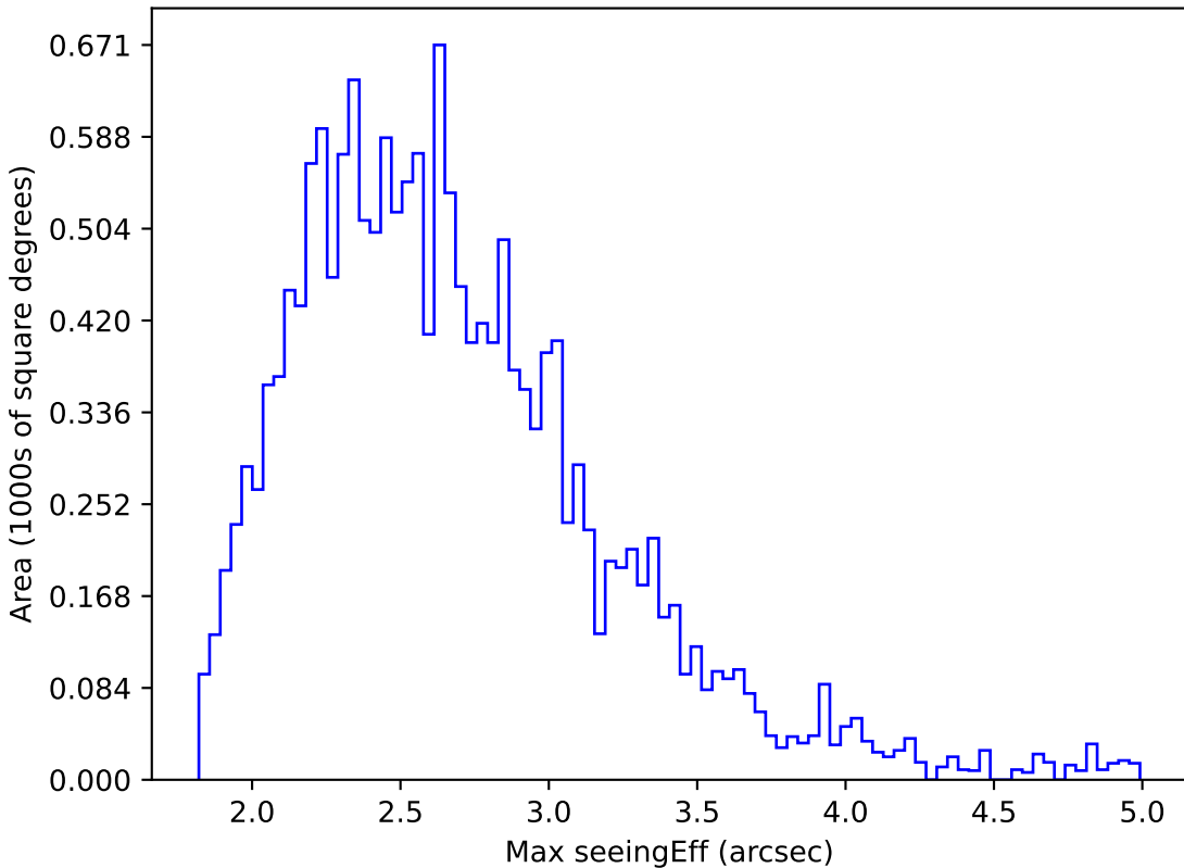
ddf_loaded_fl15_v3.4_10yrs WFD r band: Max seeingEff
