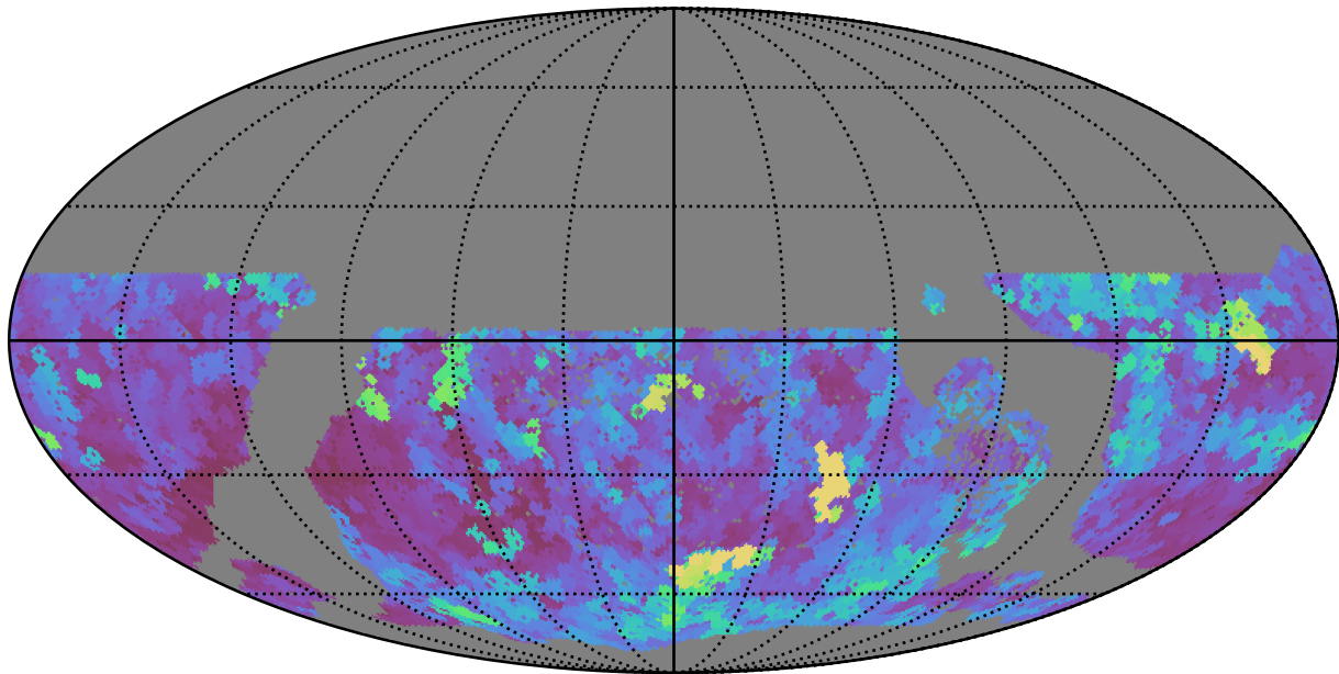
ddf_loaded_fl15_v3.4_10yrs WFD i band: Max seeingEff
