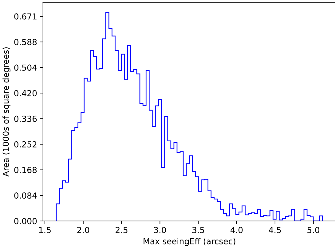
ddf_loaded_fl15_v3.4_10yrs WFD i band: Max seeingEff
