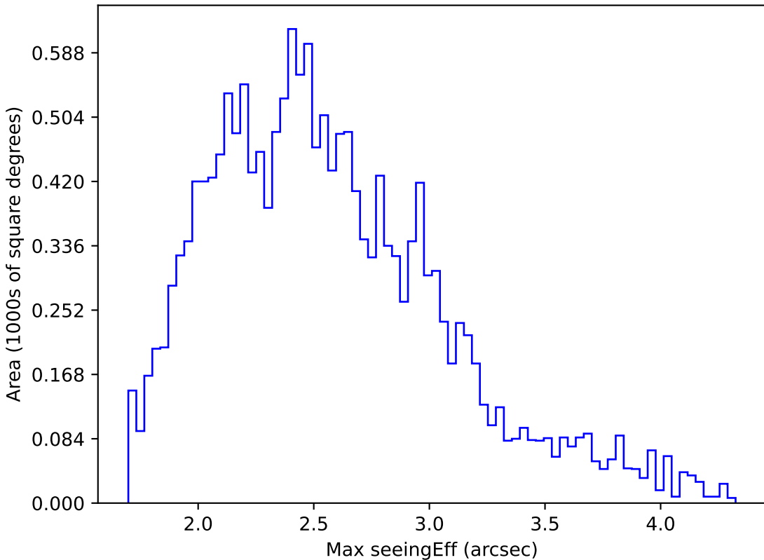
ddf_loaded_fl15_v3.4_10yrs WFD g band: Max seeingEff
