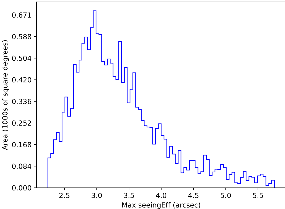
ddf_loaded_fl15_v3.4_10yrs WFD all bands: Max seeingEff
