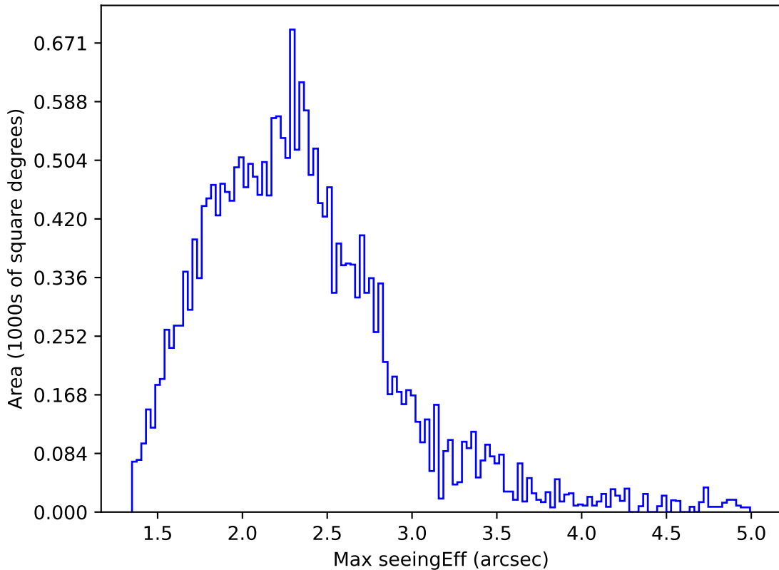
ddf_loaded_fl15_v3.4_10yrs All sky y band: Max seeingEff
