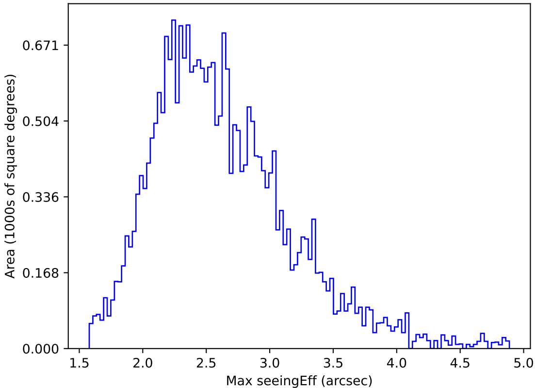
ddf_loaded_fl15_v3.4_10yrs All sky r band: Max seeingEff
