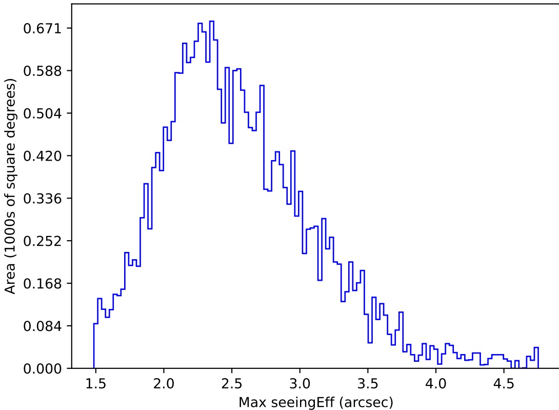
ddf_loaded_fl15_v3.4_10yrs All sky i band: Max seeingEff
