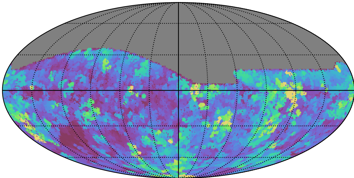
ddf_loaded_fl15_v3.4_10yrs All sky g band: Max seeingEff
