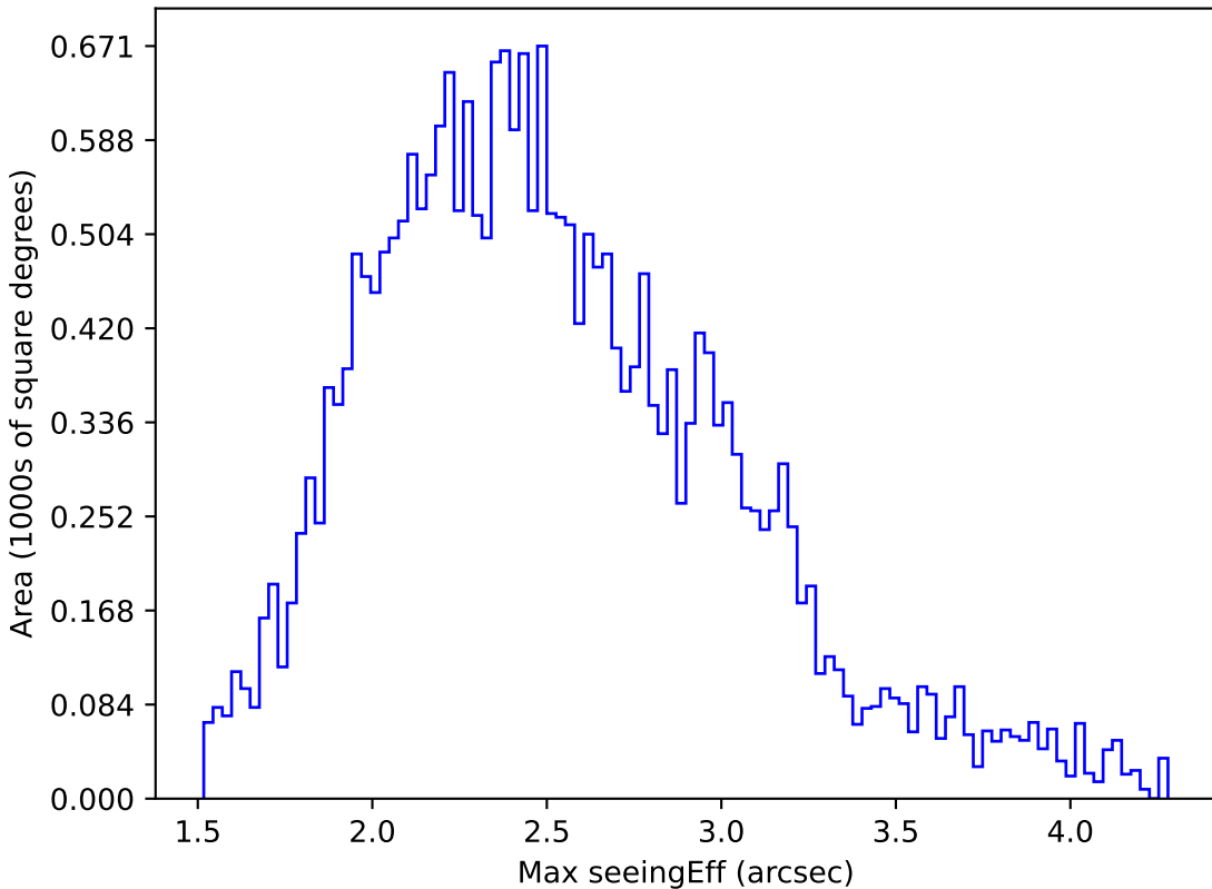
ddf_loaded_fl15_v3.4_10yrs All sky g band: Max seeingEff
