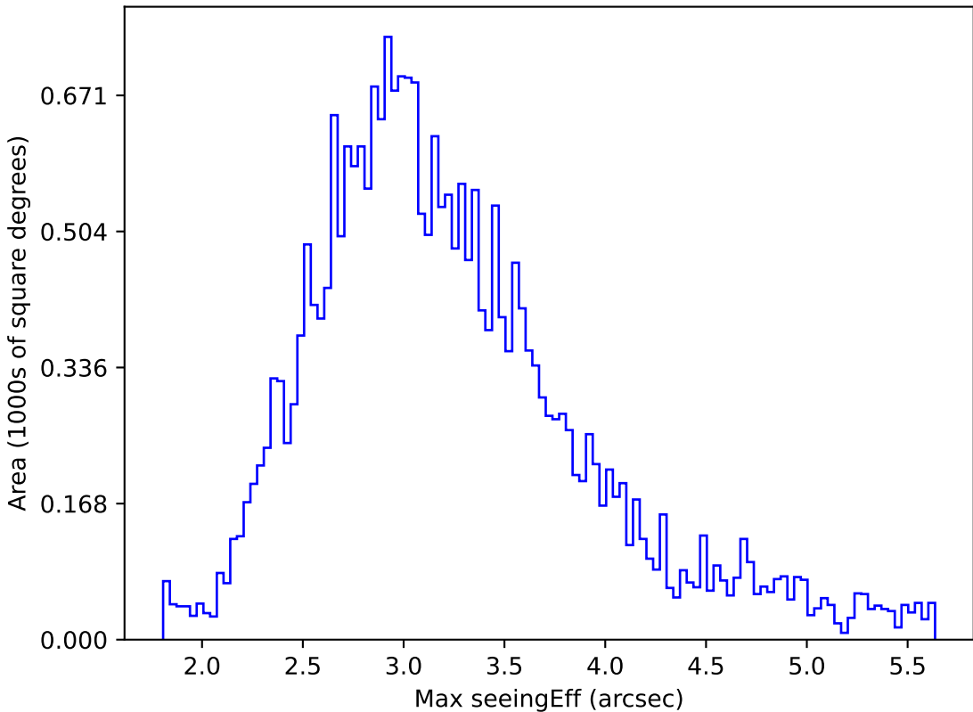
ddf_loaded_fl15_v3.4_10yrs All sky all bands: Max seeingEff
