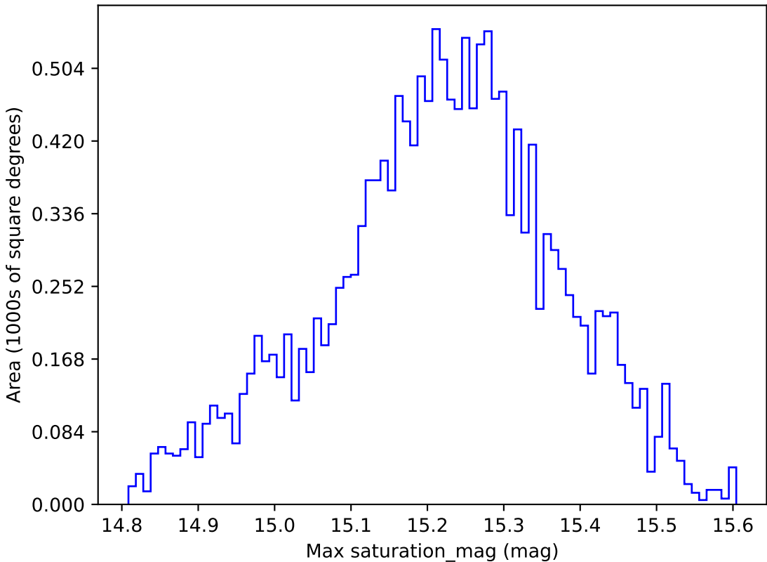
ddf_loaded_fl15_v3.4_10yrs WFD z band: Max saturation_mag
